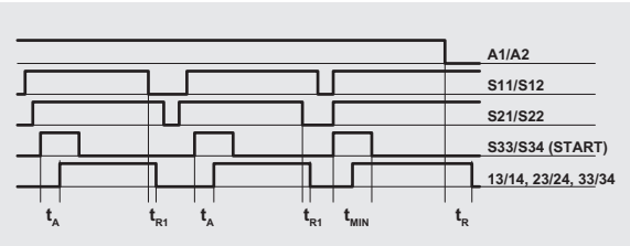
Configuration with manual start
